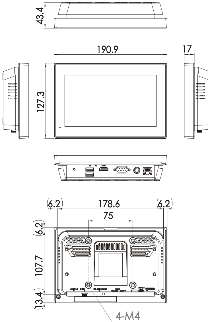
Figure 1-5: Dimensions (mm)
