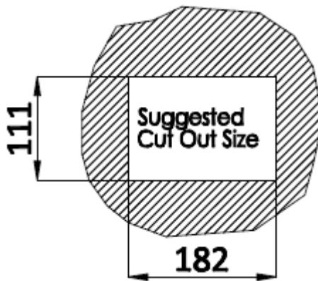
Figure 3-11: Cutout Dimensions
